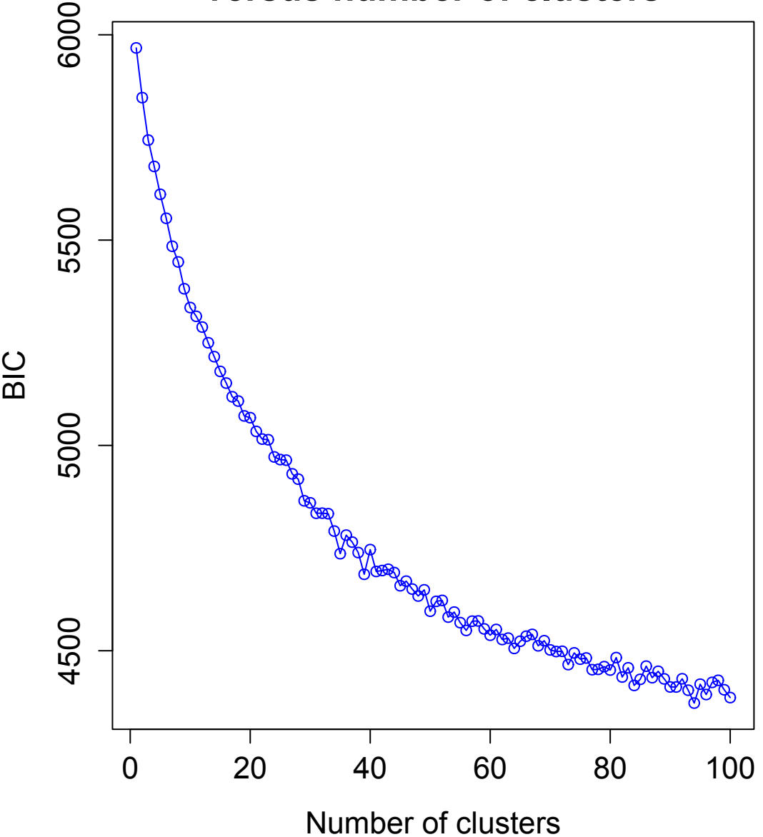
Value of BIC versus number of clusters
