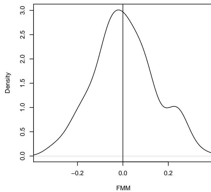
b) (h2real-h2estimated) [p=0.43]
