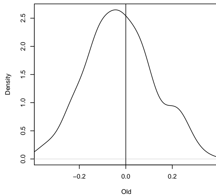
b) (h2real-h2estimated) [p=0.02]
