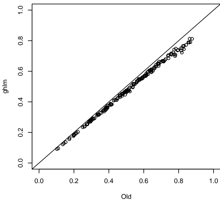
a) H2 estimates comparison
