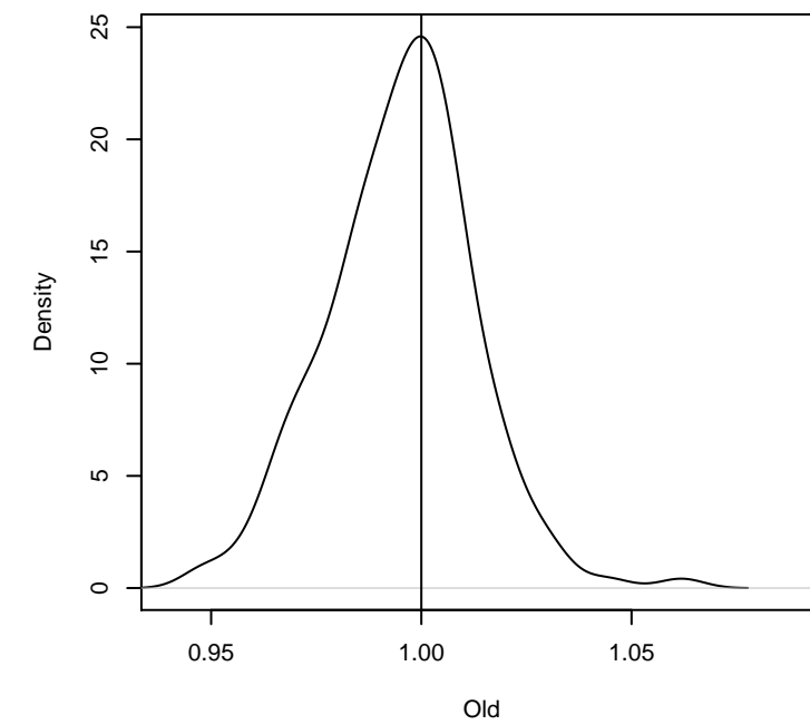
d) Lambda [p=0.00029]
