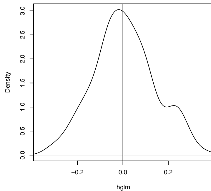
b) (h2real-h2estimated) [p=0.42]
