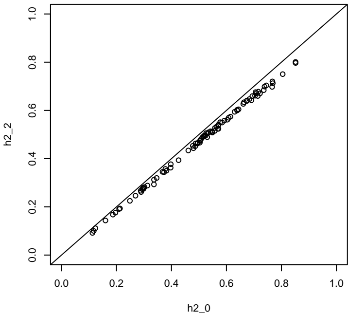
a) H2 estimates comparison
