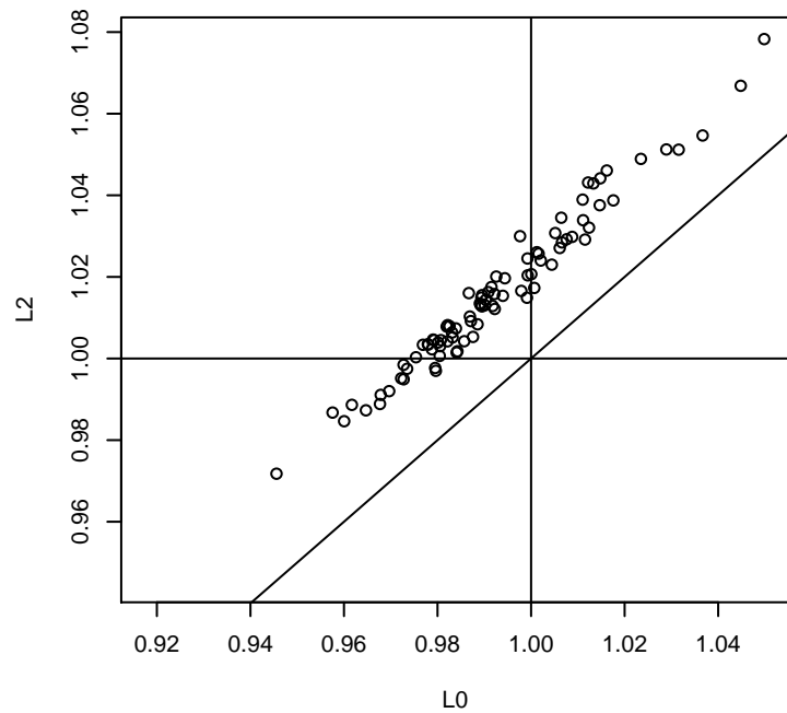
c) Lambda comarison
