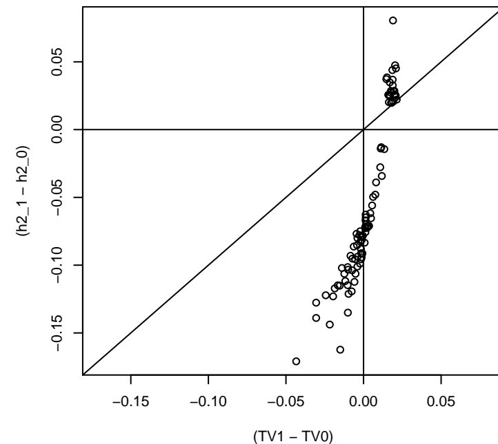
e) tVar ets diff vs. h2 ets diff
