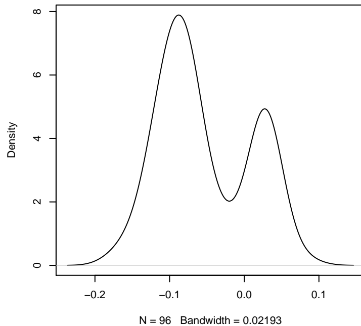
c) Density of (h2New-h2Old)
