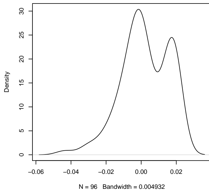
d) Density of (tVarNew-tVarOld)
