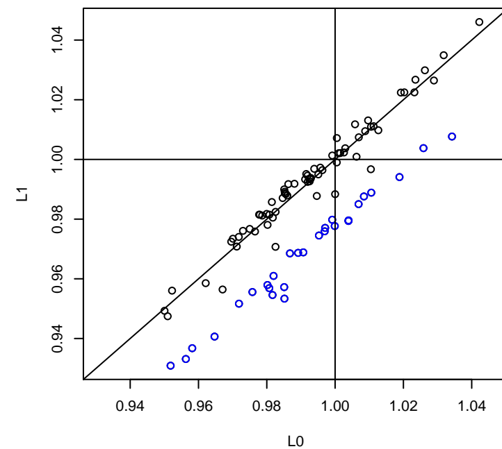
f) Lambda comarison (blue: (h2New-h2Old)>0)
