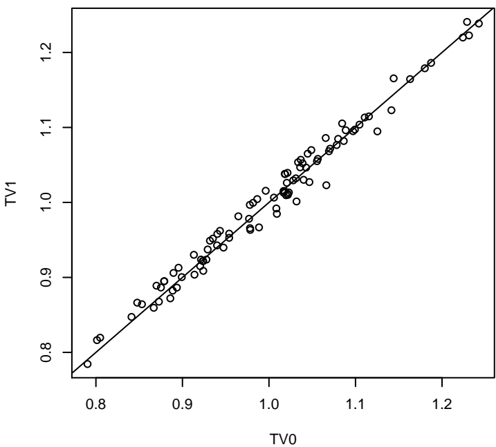
b) totVar estimates comparison
